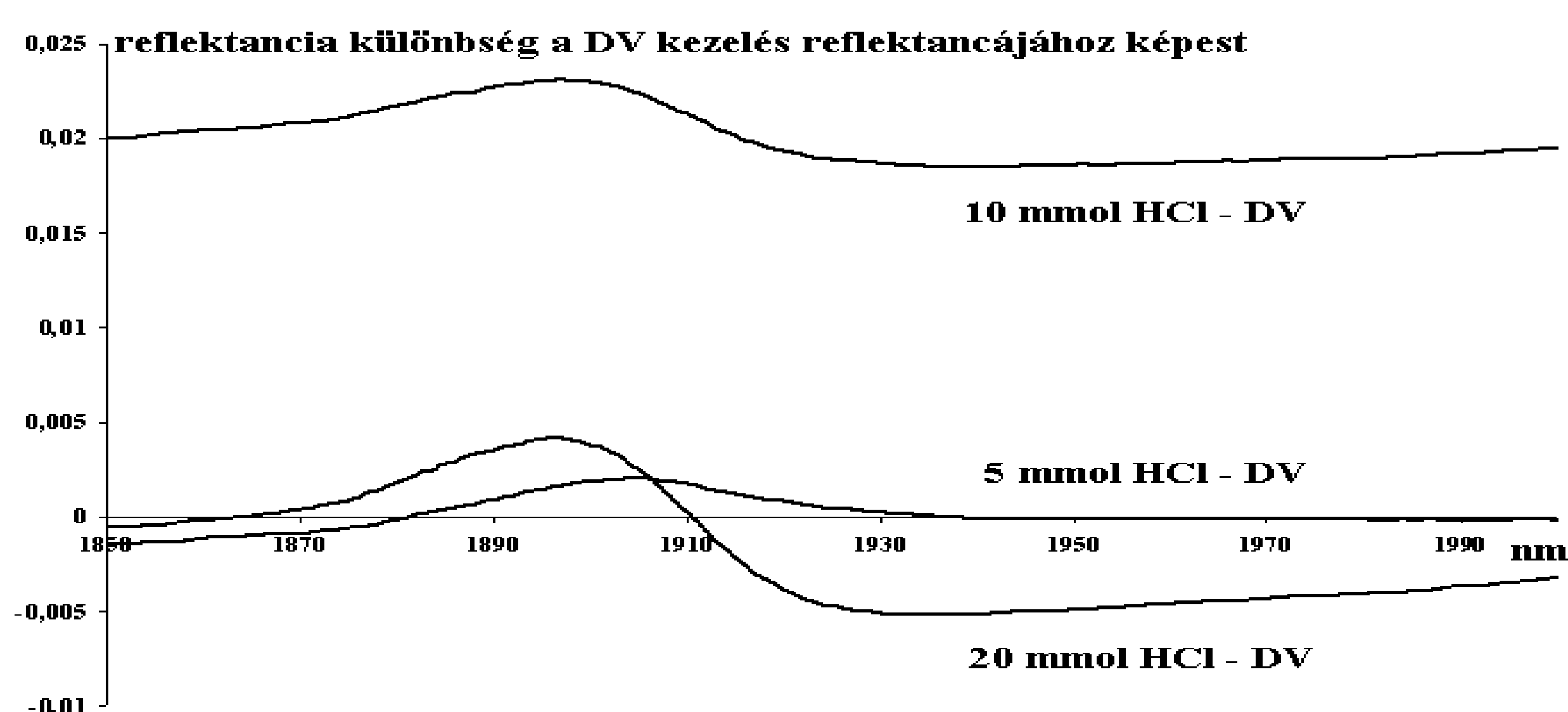
Figure 4. The informative segment of difference spectrums regarding the control treatment's spectrum
