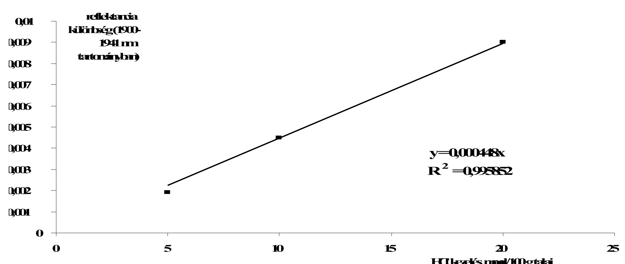
Figure 5. Correlation between the treatments and the reflectance spectrums between 1900 and 1941 nm
