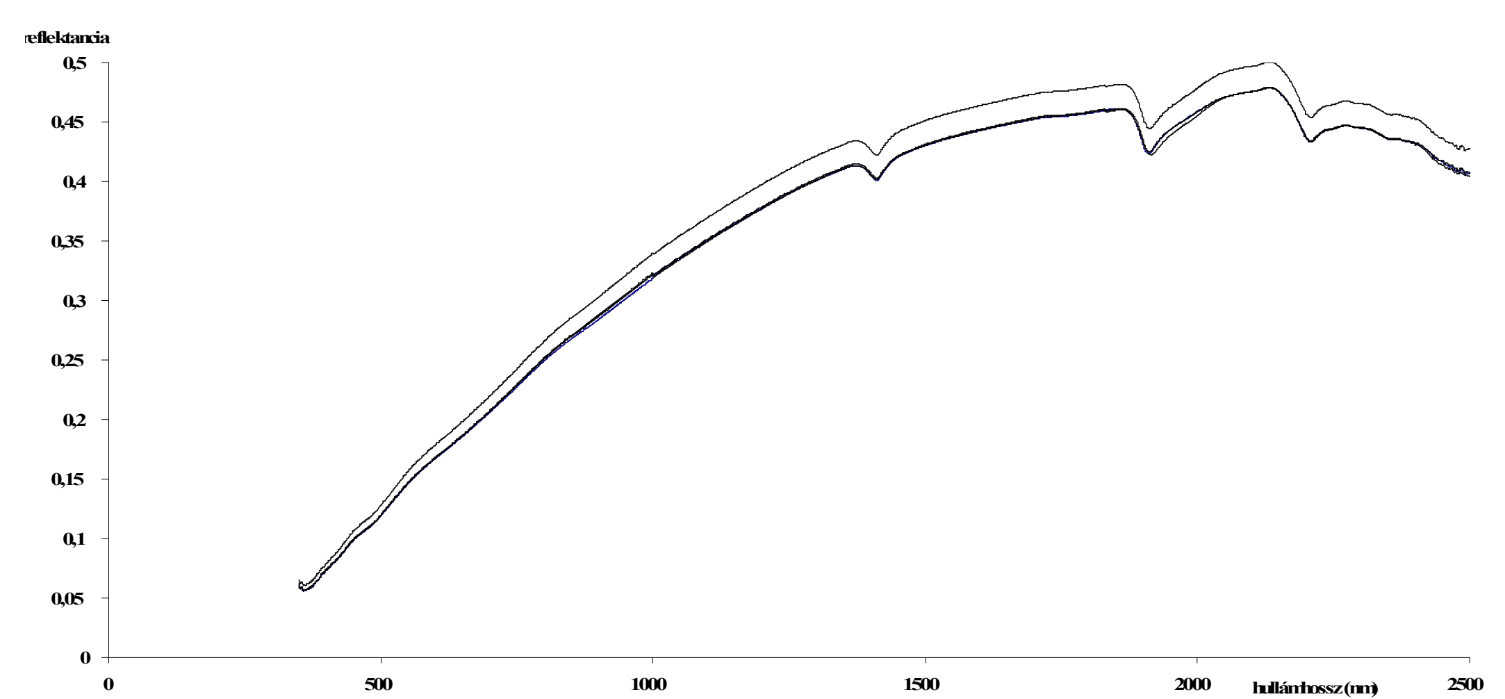
Figure 3. Means of the recorded reflectance curves resulted by various hydrochloric acid treatments. (The lower curve represents the 0, 5 and the 20 mmol, while upper represents 10 mmol acid treatments)
